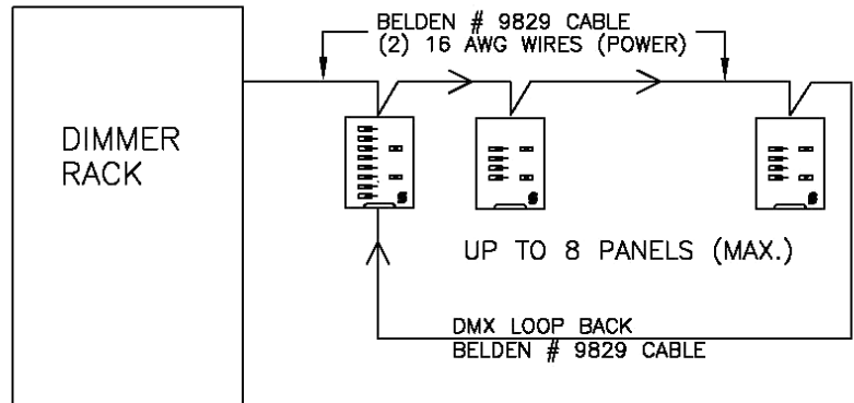
TYPICAL RISER FOR UP TO EIGHT STATIONS
